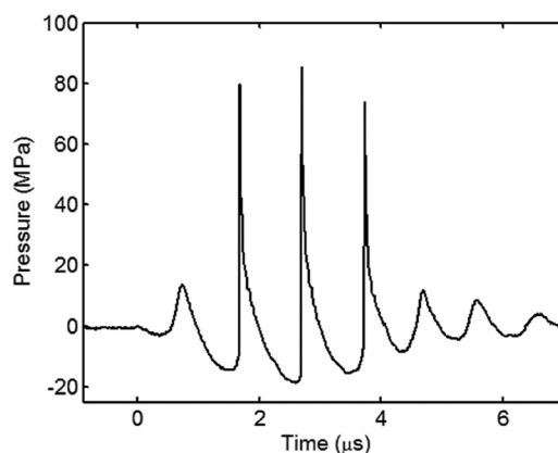
FIG. 2. A 3-cycle focal pressure waveform of the histotripsy transducer used to generate bubble clouds. The waveforms are asymmetric with a larger positive-pressure excursion than negative-pressure excursion as a result of nonlinear acoustic propagation and diffraction. Pulse lengths of 5–20 cycles were used in this study for generating clouds.
